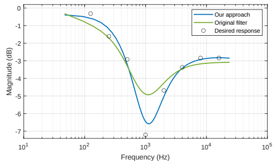
Figure 6: Absorption coefficients converted to reflectance in dB of a cotton carpet (black circles) compared with corresponding frequency responses of the filter obtained with our design approach (blue) and with filter coefficients reported in [14] (green).
